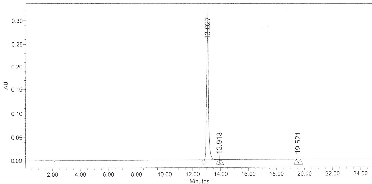
Auto-Scaled Chromatogram
